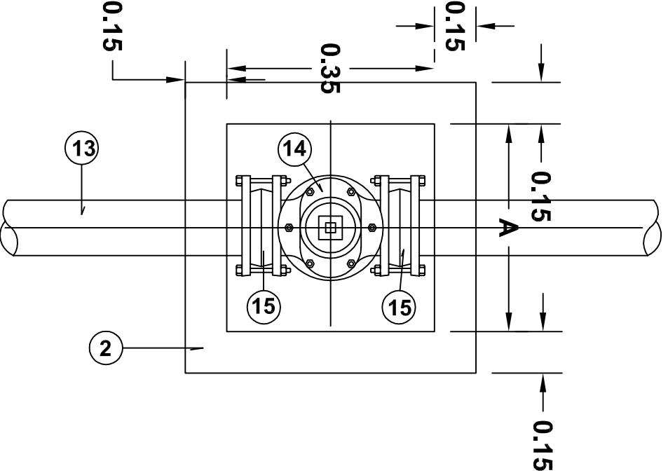
VALVULAS DIAMETROS 75 A 175mm A= 0.35m
